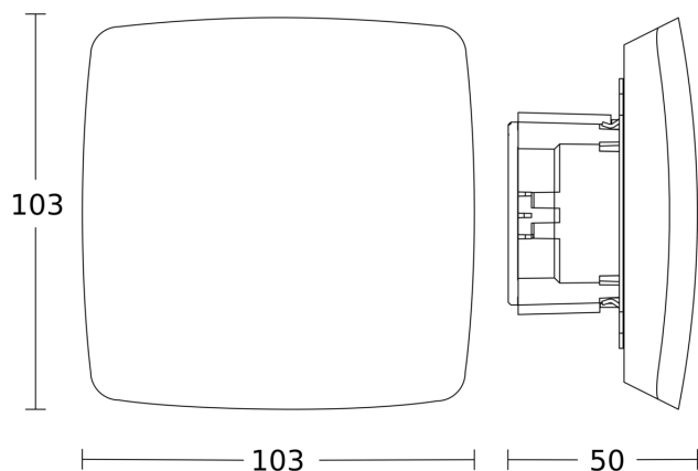
Dimension Drawing 1
